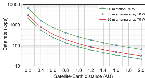
Figure 9 The data transmission rate as a function of the distance between the spacecraft and Earth. Different lines show the rate for the telescope with different size and different power.
