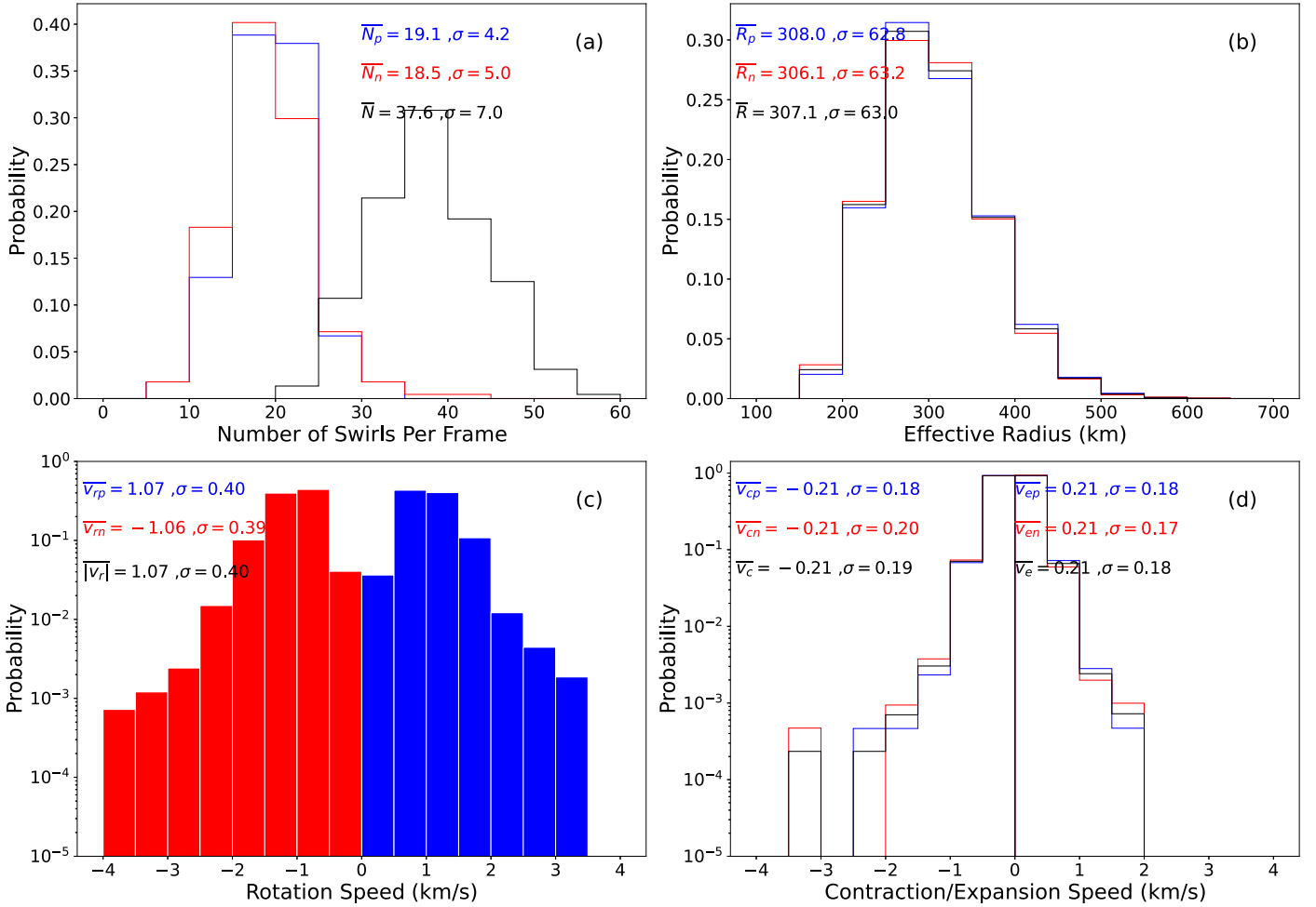
Figure 3. Statistics of the number per frame ( N ), effective radius ( R ), rotation speed ( v_r ), and contraction/expansion ( v_c/v_e ) speed of all 8424 photospheric swirls detected by ASDA from the SST Fe I 630.25 nm wide-band observation from 08:23:36 UT to 08:39:18 UT on 2019 July 7. Subscripts p and n (blue and red) denote positive and negative swirls, respectively. \sigma in each frame is the corresponding standard deviation.
