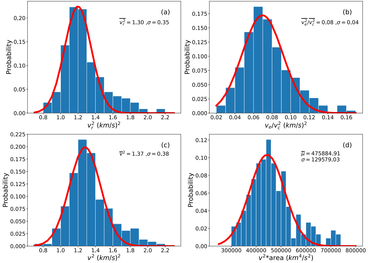
Figure 7. Statistics of the square of rotation speed ( v_r^2 ), the square of contraction/expansion ( v_e/v_c^2 ) speed, the square of speed ( v^2 ) and the product of the square of speed ( v^2 \cdot \text{area} ), and area of all 8880 photospheric swirls detected by ASDA from the SST Fe I 6302 Å wide-band observation from 08:23:36 UT to 08:39:18 UT on 2019 July 7. Red lines represent fitted Gaussian curves.
