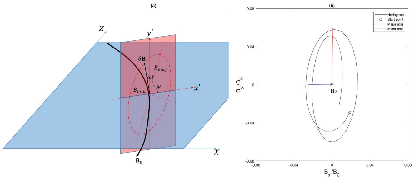
Figure 8. (a) illustration of the elliptically polarized \delta\mathbf{B}_\perp components. The blue plane is the simulation plane, and the red plane is the plane perpendicular to local background magnetic field \mathbf{B}_0 . y' axis is perpendicular to simulation plane, and x' axis is perpendicular to \mathbf{B}_0 while lies in the simulation plane; (b) hodogram of \delta\mathbf{B}_\perp at x = 5.205R_E , y = 0.457R_E during 128.5\Omega_p^{-1} < t < 151.5\Omega_p^{-1} . The black circle marks the start point of the hodogram, and the blue and red lines mark the direction of minor and major axes, respectively. The direction of background magnetic field is out of page.
