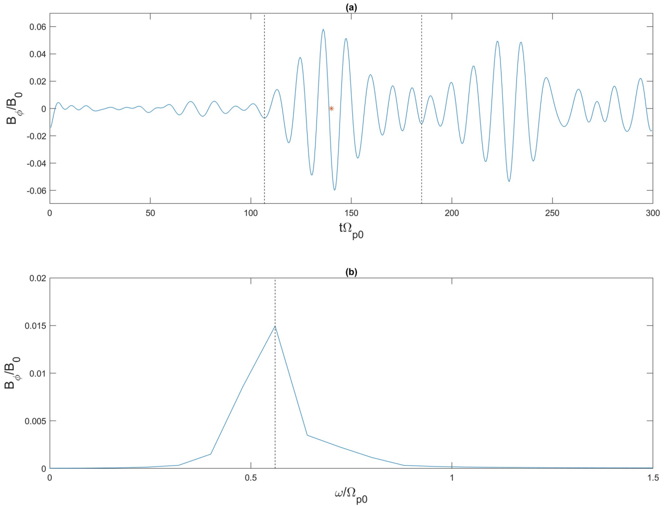
Figure 4. (a) Temporal evolution of B_\phi at location x = 5.205R_E , y = 0.457R_E . The red star marks the time t = 140\Omega_{p0}^{-1} at which the wave packet pass through the location, and the two black dashed lines marks the time interval during which the wave packet propagates through this point; (b) wave spectrum of the wave packet in (a). The spectrum peaks at \omega = 0.5567\Omega_{p0} .
