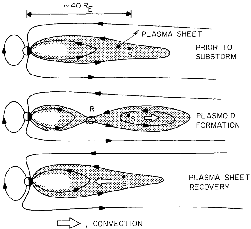
Figure 2. Plasmod model for magnetotail substorms.
