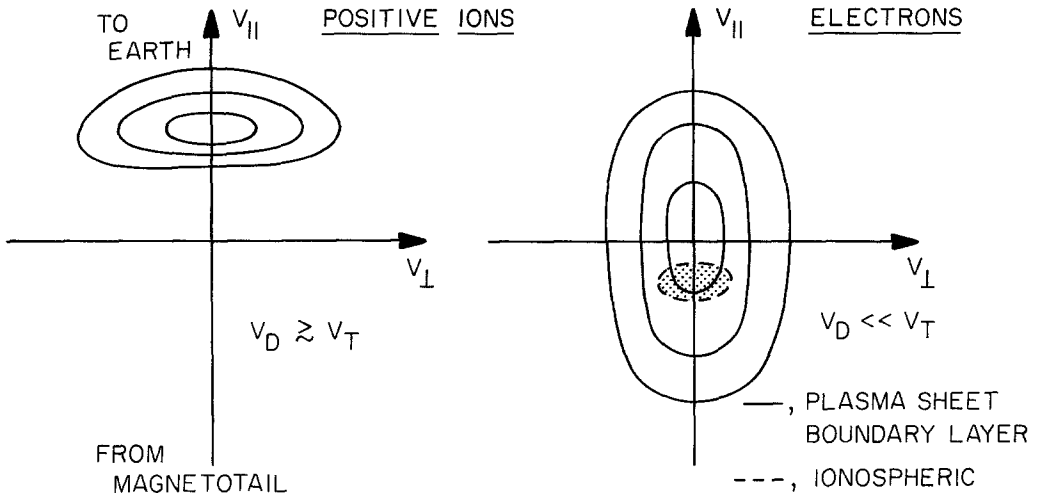
Figure 3. Ion and electron velocity distributions in the plasma sheet boundary layer.
