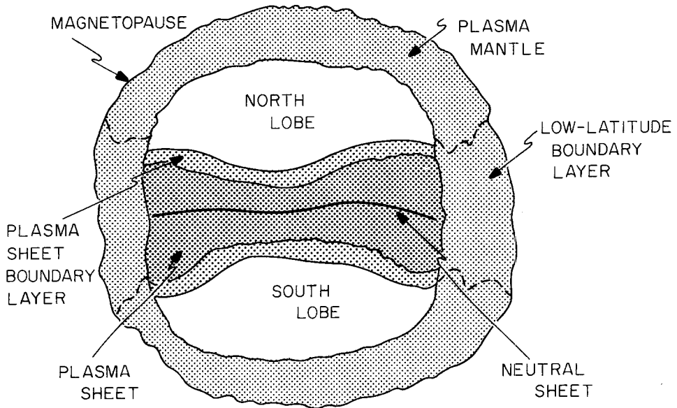
MAGNETOTAIL CROSS-SECTION AT \sim 40 R_E
