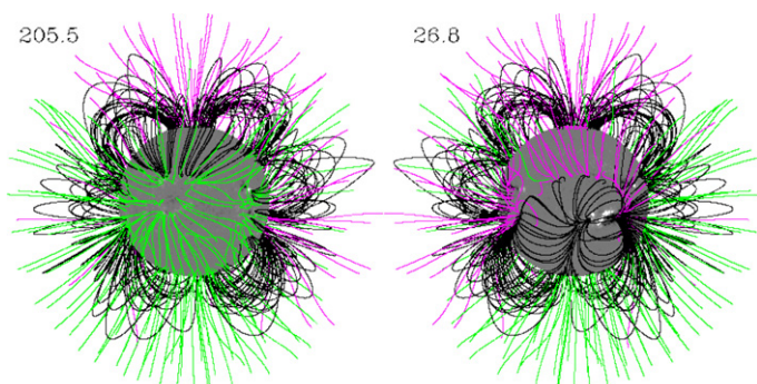
Figure 6. Coronal magnetic field topologies obtained from the SSW PFSS model, with central longitudes being 205^{\circ}5' (left) and 26^{\circ}8' (corresponding to the Carrington times of 2004 July 6 20:00 and July 20 08:00). The closed field lines are colored black, and the open outward (inward) field lines are represented with purple (green) lines.
