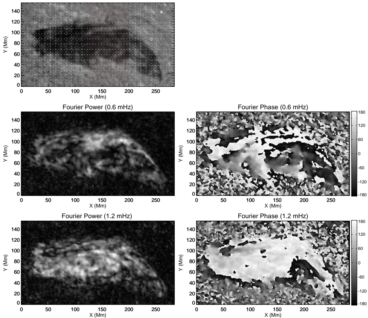
FIG. 7.— Oscillation of the filament F1. Top: dotted lines indicate the central positions of the slits used in Figure 8 and Figure 9. The lines in red show the central positions of the slits along which the filament material oscillated coherently. Middle and bottom panels show the Fourier power (left) and phase (right; ranging from -\pi to \pi ) at 0.6 and 1.2 mHz, respectively. An animation of the cutout H\alpha images is available in the electronic version of the Journal.
