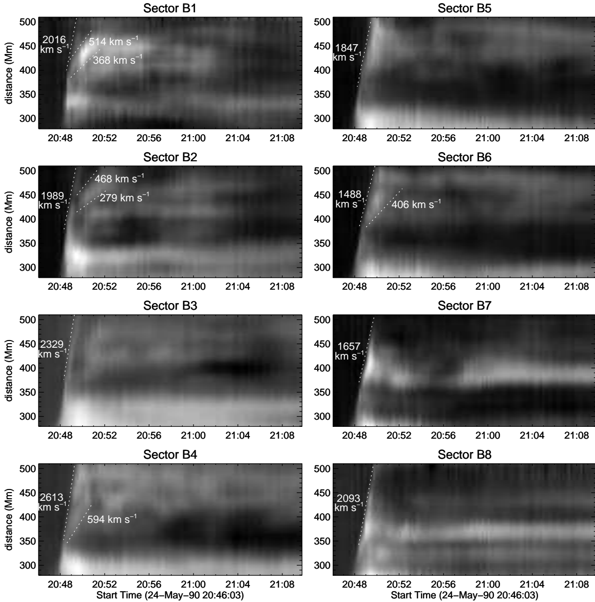
FIG. 6.— Space-time plots showing the propagation of the Moreton wave as observed by the BBSO 10-inch telescope. The plots are obtained by integrating across each individual sector in Figure 2(a) along the azimuthal direction and subtracting the initial profile (see the text). Dotted lines show linear fits of visually picked points along the tracks left by the fast wavefront as well as a slow, diffuse front.
