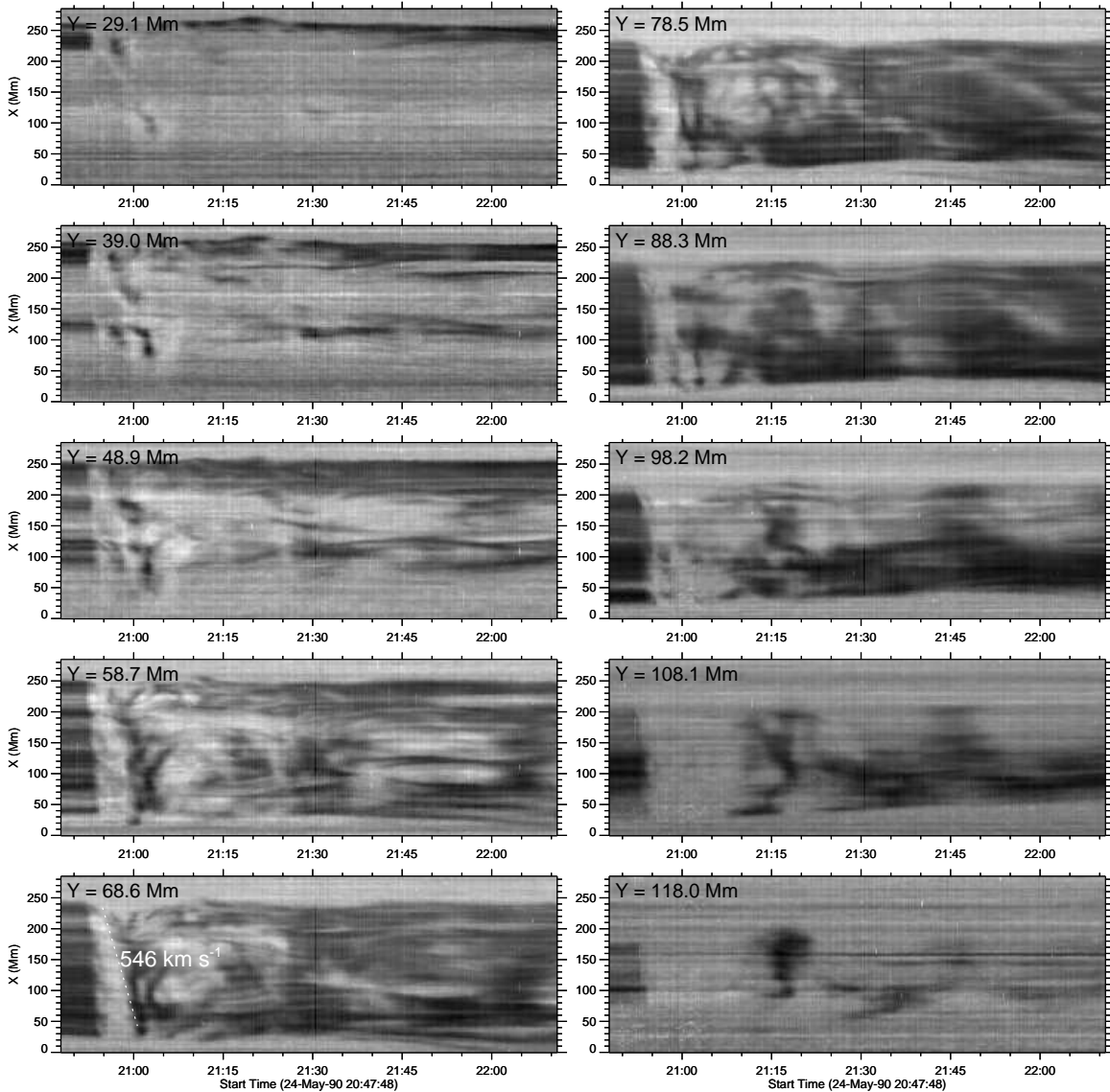
FIG. 8.— Evolution of F1 seen through the east-west oriented slits in the top panel of Figure 7. In the stack plot obtained with the horizontal slit at Y = 68.6 Mm, the dotted line show a linear fit to visually picked points along a inclined dark feature.
