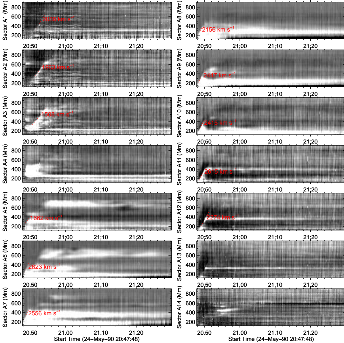
FIG. 5.— Space-time plots showing the propagation of the Moreton wave as observed by the BBSO 8-inch telescope. The plots are obtained by integrating across each individual sector in Figure 4 along the azimuthal direction and subtracting the initial profile (see the text). Dotted lines show linear fits of visually picked points along the tracks left by the wavefront. The slope of each track indicate the speed of the wavefront.
