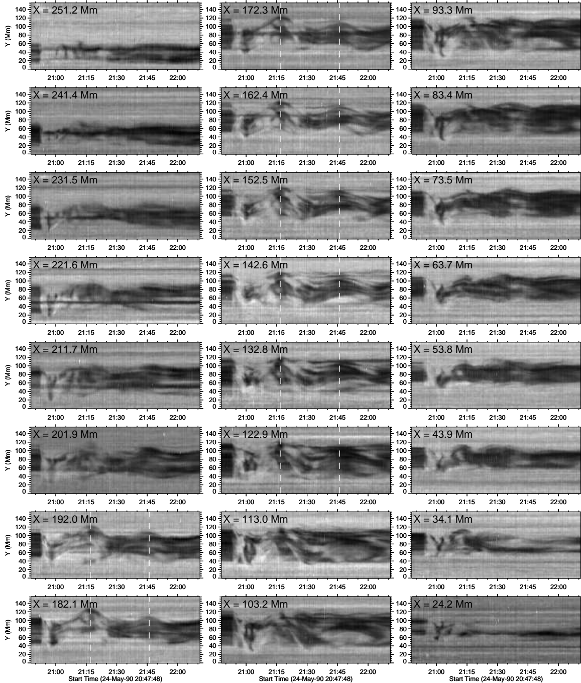
FIG. 9.— Evolution of F1 seen through the north-south oriented slits in the top panel of Figure 7. Dashed lines mark the peaks of a sine-like pattern.
