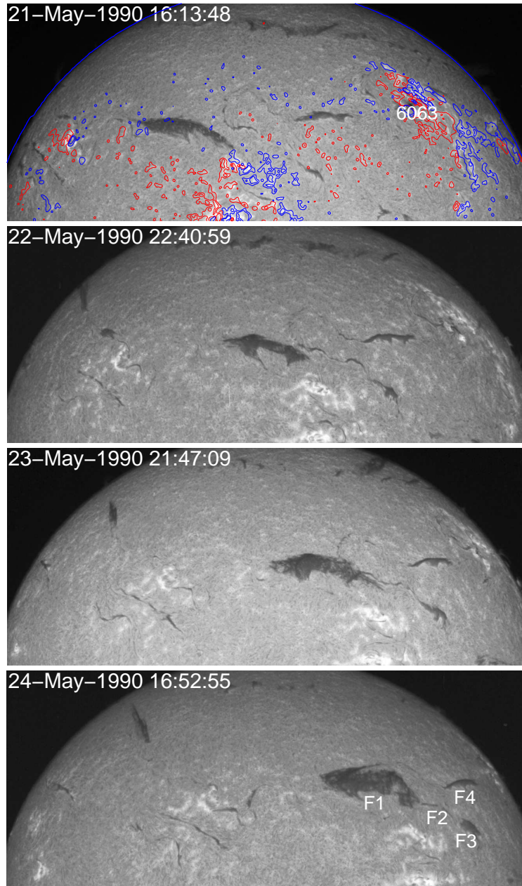
FIG. 11.— Evolution of the filaments of interest from 1990 May 21 till 24, prior to the initiation of the Moreton wave. The top panel is overlaid by a magnetogram taken at approximately the same time at Kitt Peak by National Solar Observatory. The contours show the line-of-sight component of the photospheric field at levels of \pm 200 , \pm 50 G, with red (blue) colors indicating positive (negative) polarities.
