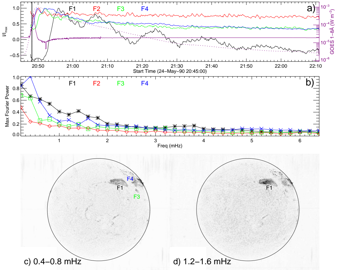
FIG. 3.— Filament oscillation driven by the Moreton wave. a) Lightcurves of the filaments F1-F4, color-coded according to the colors of the rectangular boxes in Figure 1(a). The curves are normalized by each own maximum and scaled by the y-axis on the left. Over-plotted are the GOES 1–8 Å flux (purple dotted line), scaled by the y-axis on the right, and its time derivative (purple solid line), shown in an arbitrary scale. b) Maximum Fourier power obtained from each individual rectangular box in Figure 1(a). c) and d) Fourier power integrated over relevant frequencies around which the curves in b) have local maxima. The colors are reversed so that enhanced features appear dark. The solar limb is indicated by the circle.
