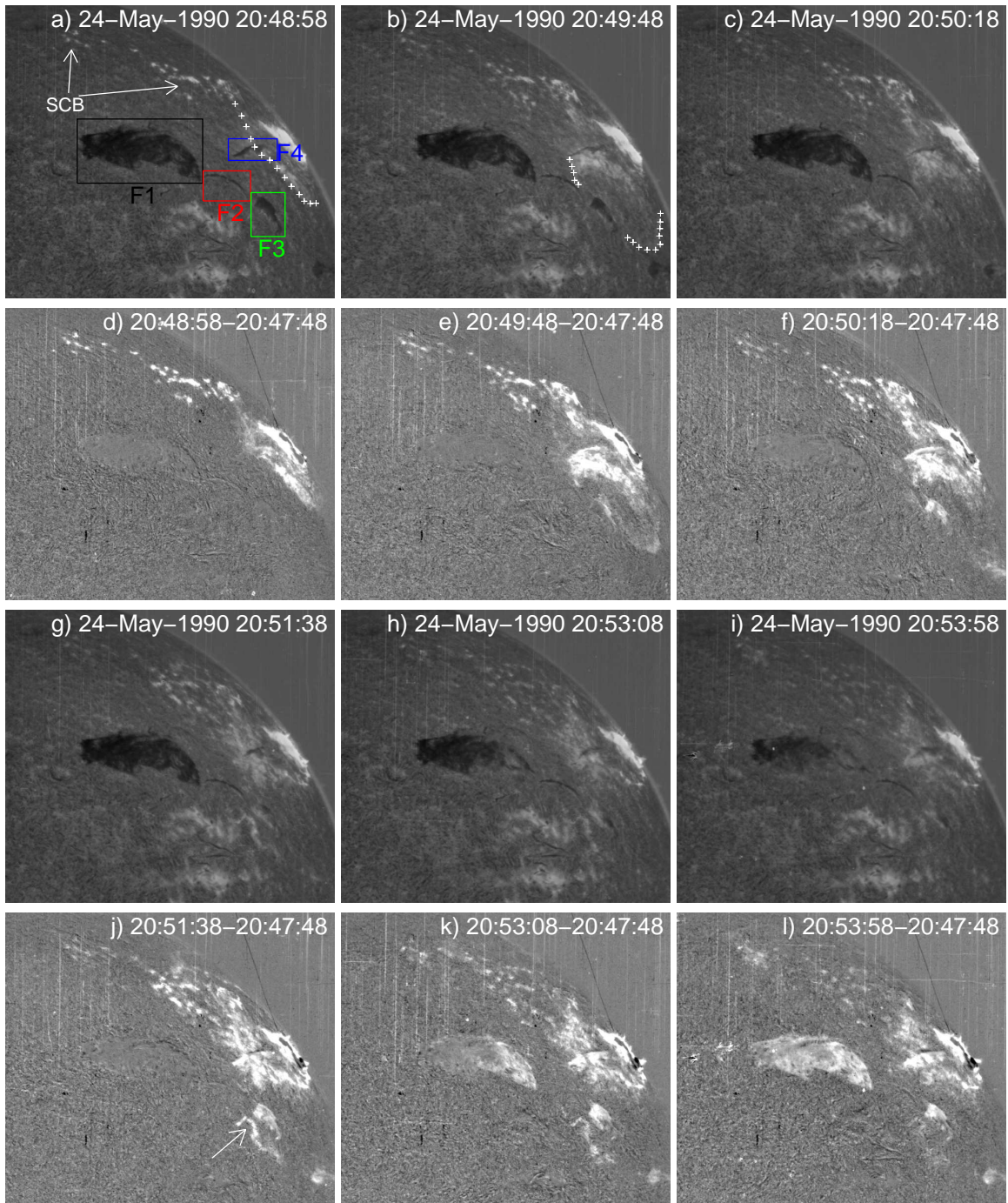
FIG. 1.— Sequence of H\alpha images showing the propagation of the Moreton wave and its interaction with the remote filaments. The initial wavefront is marked by ‘+’ symbols. The colored rectangular boxes enclose the four filaments of interest. The 2nd and 4th row show corresponding base-difference images. An animation of full-disk H\alpha images is available in the electronic version of the Journal.
