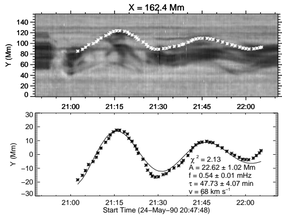
FIG. 10.— Oscillatory pattern fitted with a damped cosine function. The top panel shows the space-time evolution as seen through the N-S slit at X = 162.4 Mm (Figure 9). Visually picked points featuring the oscillatory pattern are indicated by white asterisks. After de-trended with a 2nd order polynomial, these points are fitted with a damped cosine function, i.e., A \cos(2\pi ft + \phi) \exp(-t/\tau) . The fitting results are given in the bottom panel. The velocity amplitude is obtained from the derivative of the damped cosine function.
