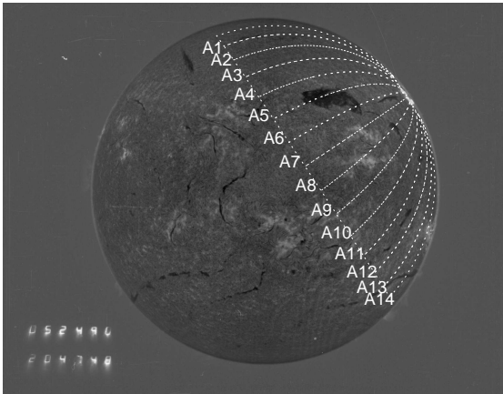
FIG. 4.— Angular sectors, A1–A14, used to track the wave propagation.
